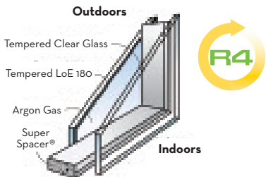
R4 Tempered LoE 180, Argon with Super Spacer®
