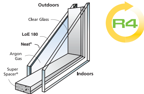
R4 LoE 180 Neat®, Argon with Super Spacer
