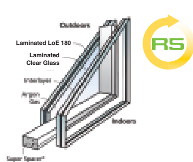
R5 (Custom Patio Door) Laminated, LoE 180, Argon with Super Spacer®
