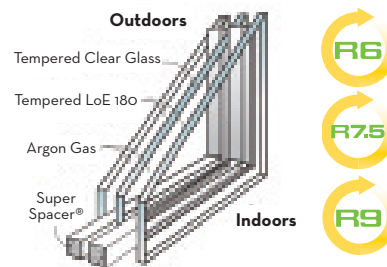
R6 Tempered Triple Pane, LoE 180, Argon with Super Spacer® R7.5 Tempered Triple Pane, LoE 180, 50% Argon / 50% Krypton with Super Spacer® R9 Tempered Triple Pane, LoE 180, Krypton with Super Spacer®
